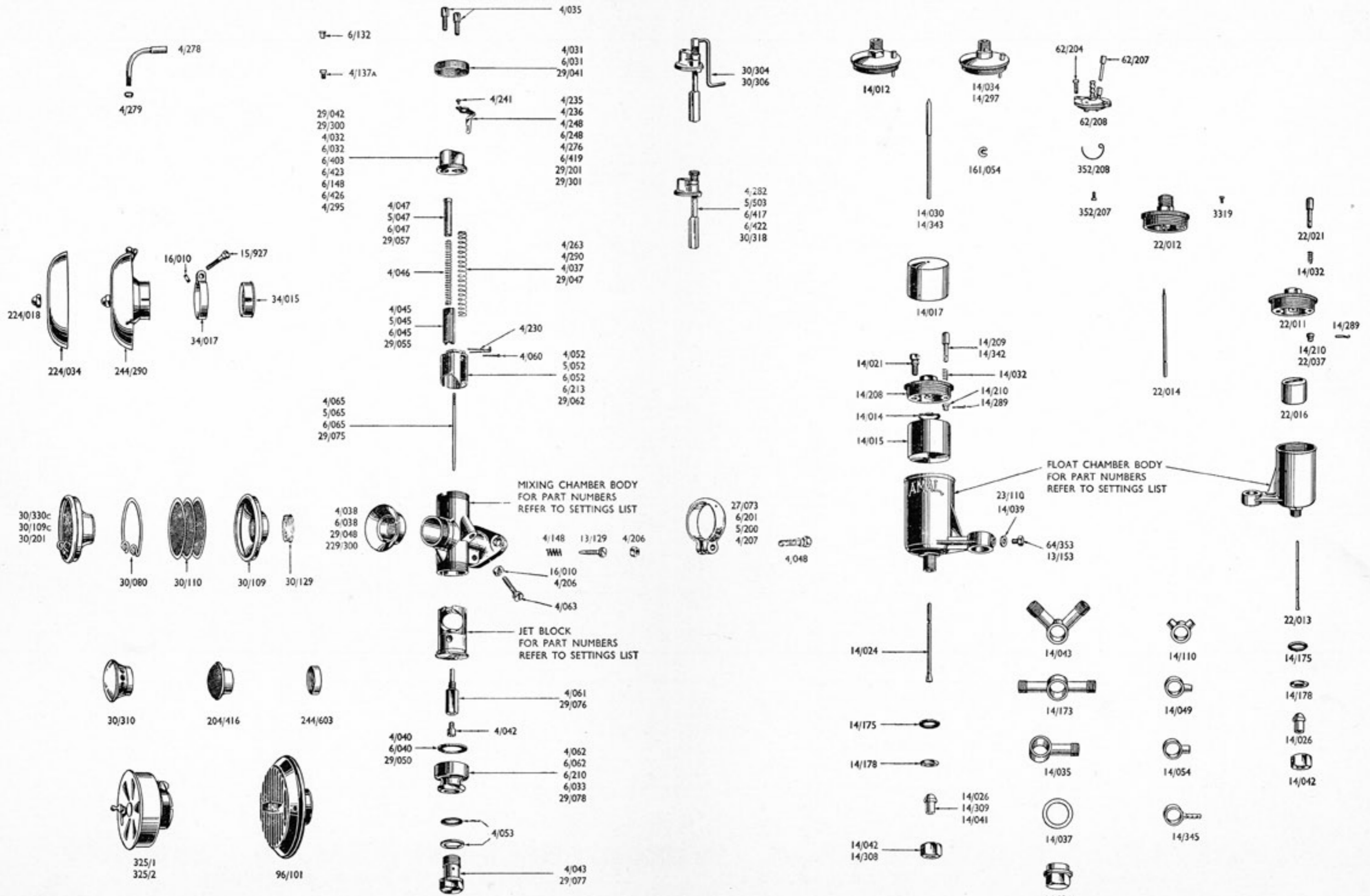
SPARE PARTS ILLUSTRATION FOR STANDARD NEEDLE TYPE CARBURETTORS
